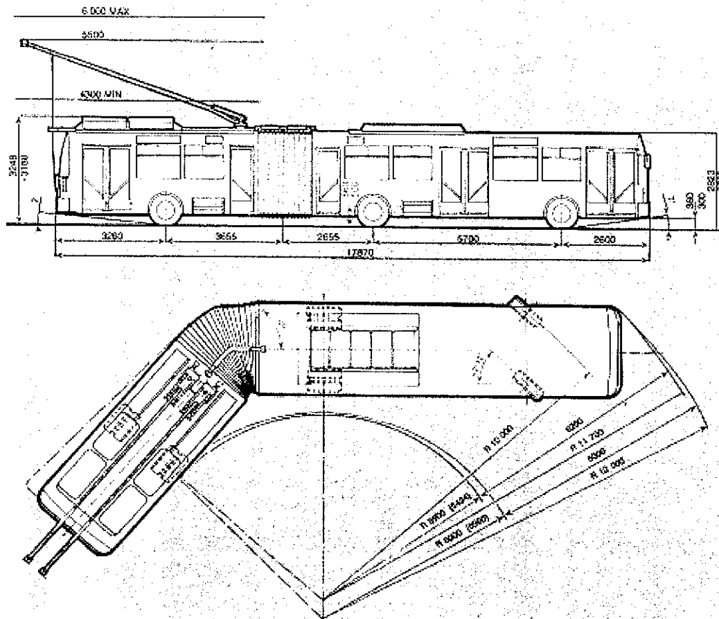
Figure 3.2.3. Dimensions of the low-floor articulated Skoda bus (22tr).
