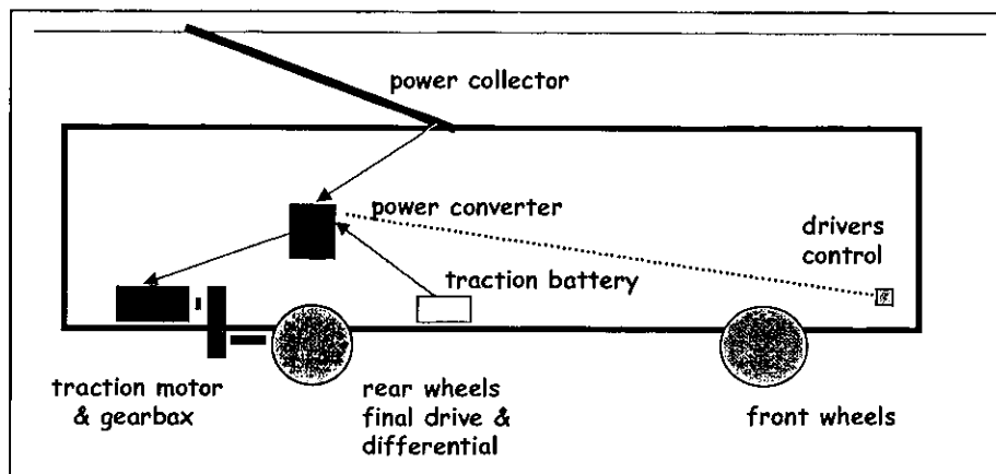
Figure 3.1.1. Principal trolley bus.
