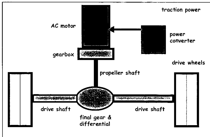
Figure 3.1.4. Principal chassis mounted motor system.
