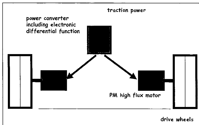
Figure 3.1.3. Principal hub motor system.
