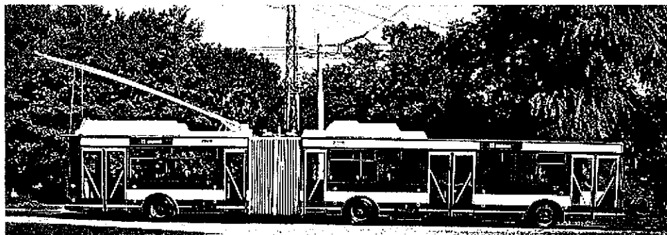
Figure 4.1.1 Skoda's low-floor articulated bus model (22tr).
