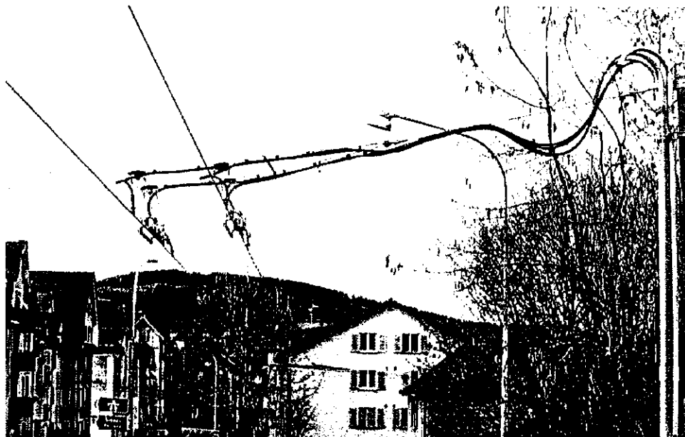
Figure 3.3.4 Feeder point with section insulator (Source: Furrer+Frey).
