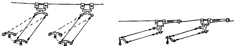
Figure 3.3.1. Pendulum system.
