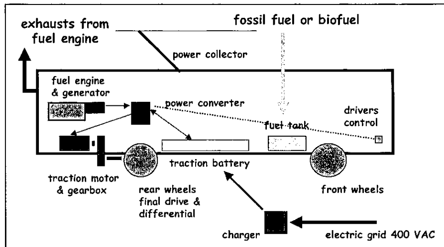
Figure 3.1.2 Principal dual mode bus.
