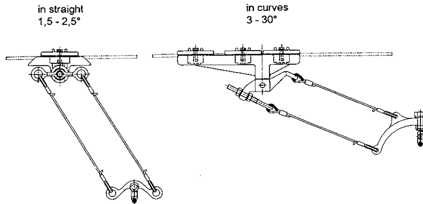
Figure 3.3.2. Suspension system from Kummler+Matter.
